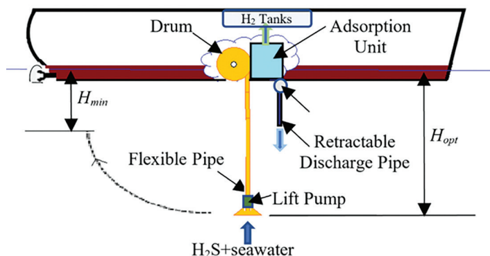
Figure 5: Flexible and retractable H_2S claim system of the mother ship. The figure is not to scale ©Birol Kilkis
